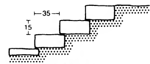
21 Block steps in natural or cast stone
